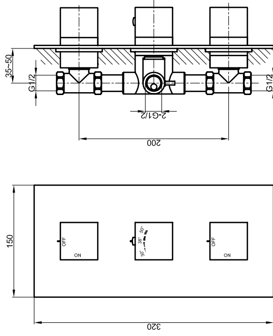
Technique drawing
