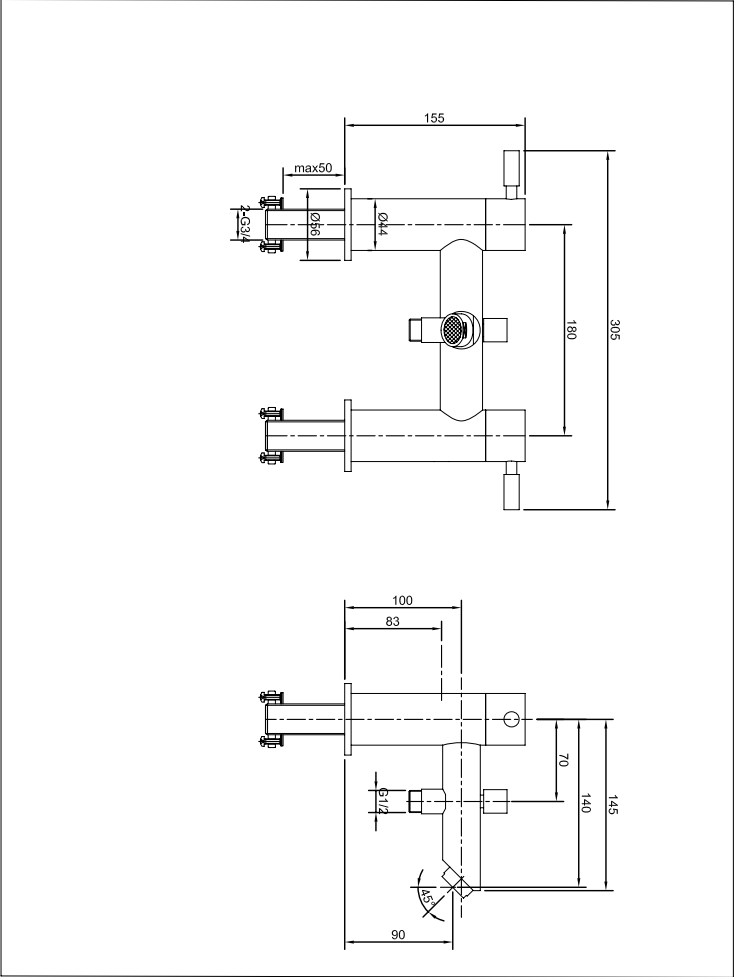
Technique drawing
